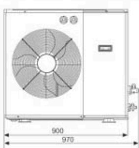
ZB30,ZB38,ZB45外形尺寸
